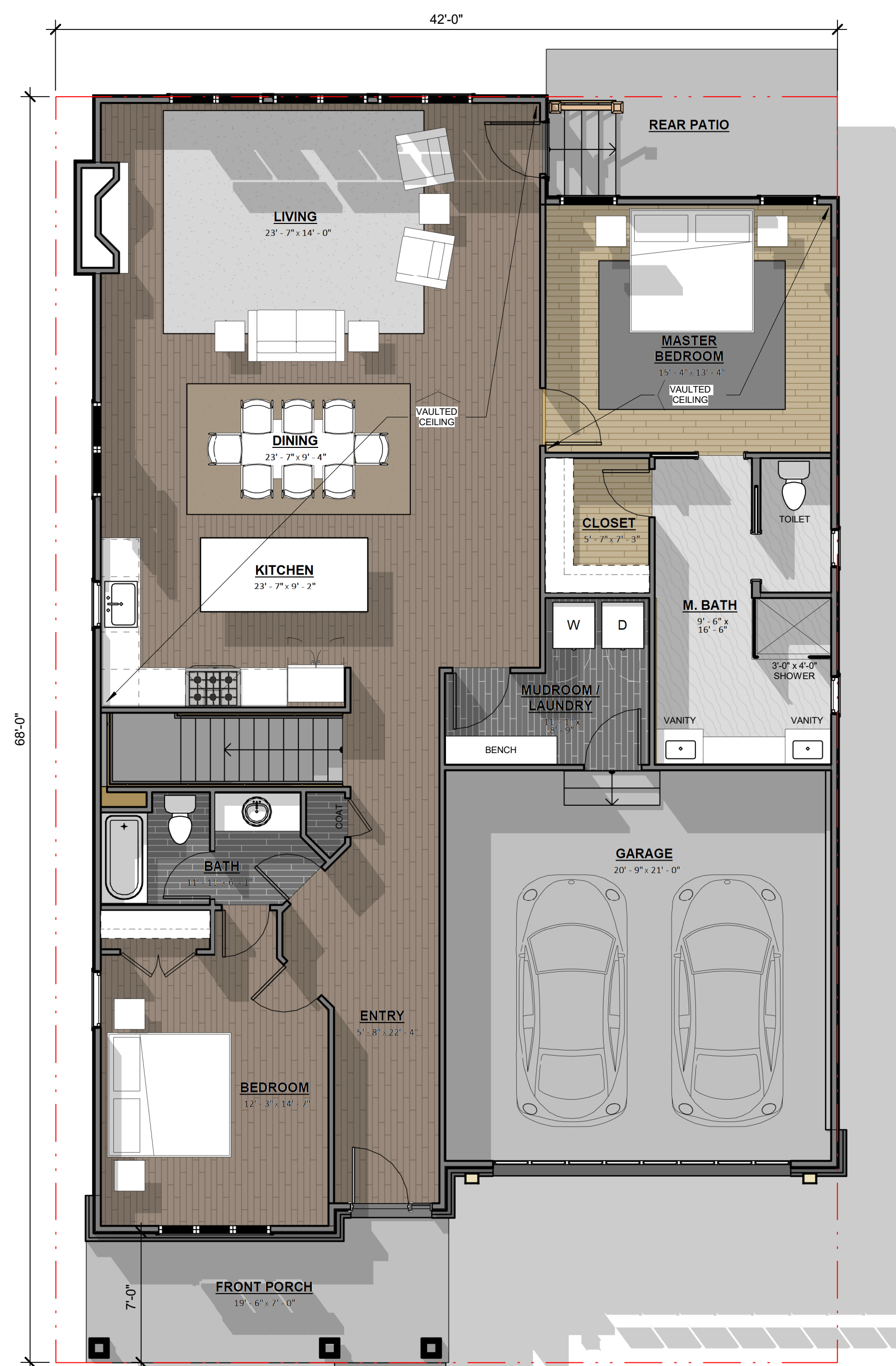
FIRST FLOOR +/-1,800 SF (+/- 460 SF GARAGE)
