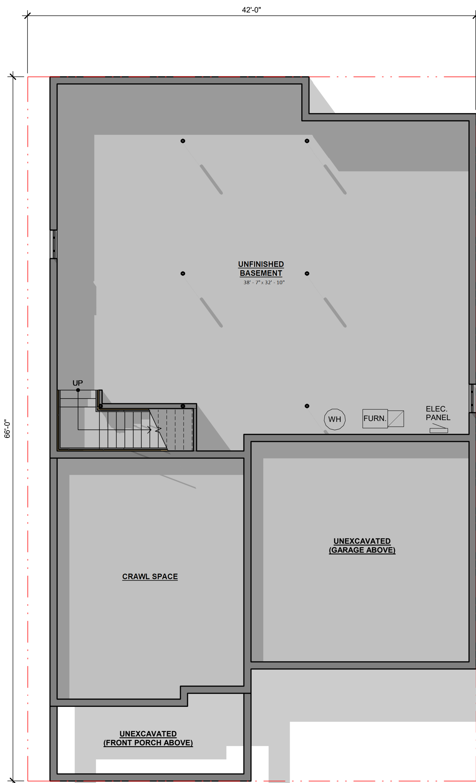
BASEMENT +/-1,350 SF
